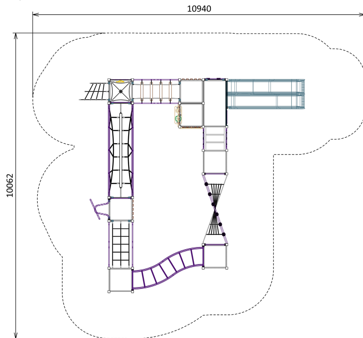
Plan View
