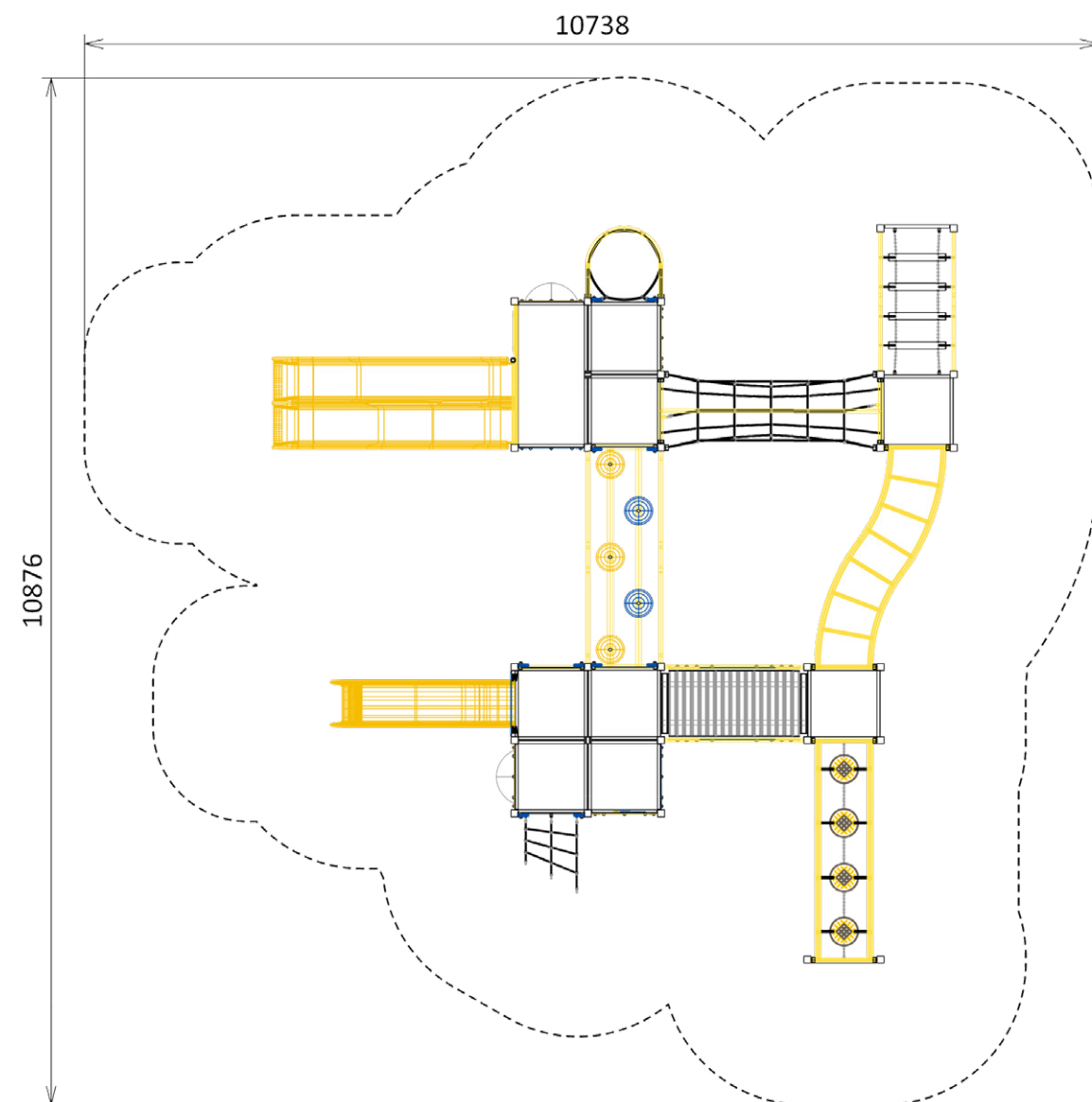
Plan View
