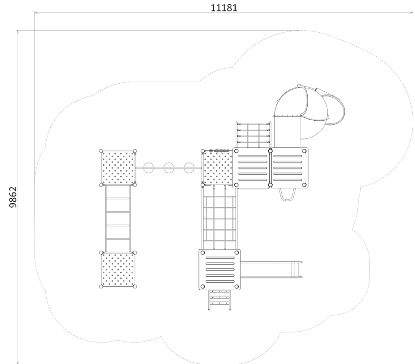
Plan view
