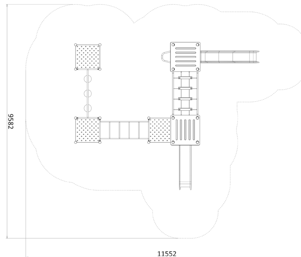
Plan View
