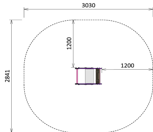
ACCESSIBLE SCUTTLE ROCKER (SE-70)
