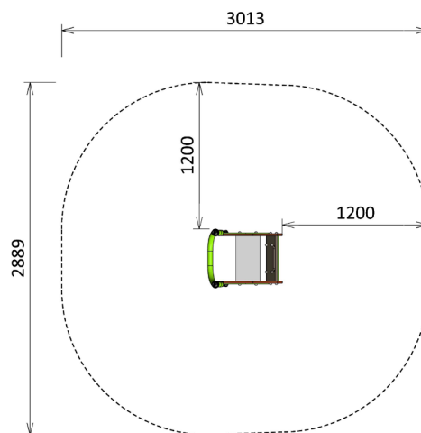
ACCESSIBLE DIPPER ROCKER (SE-71)
